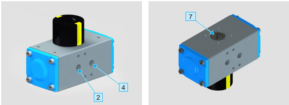
Fig. 3-2 bar-acturn GD-032 overview of components (left: top view, right: bottom view)
