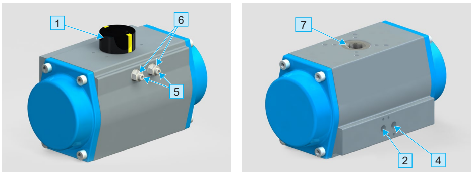
Fig. 3-3 bar-acturn GD/GS-125 overview of components (left: top view, right: bottom view)
