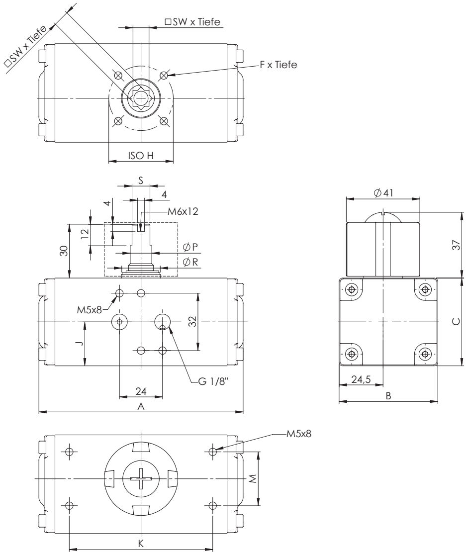
Fig. 13-1 Dimensional drawing bar-agturn type GD-032
