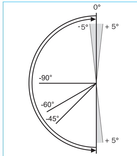
Fig. 6-2 Adjustable mechanical swivel angle range of the bar-acturn version 120°/135°/180° from size GD-040, GD/GS-052 till 210
