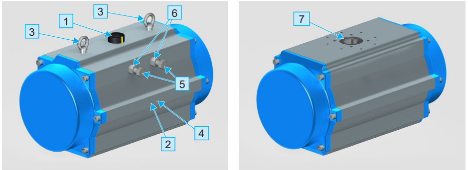
Fig. 3-4 bar-agturn GD/GS-300 overview of components (left: top view, right: bottom view)
