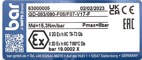
Fig. 3-5 Type plate of single-acting and double-acting rotary actuator
