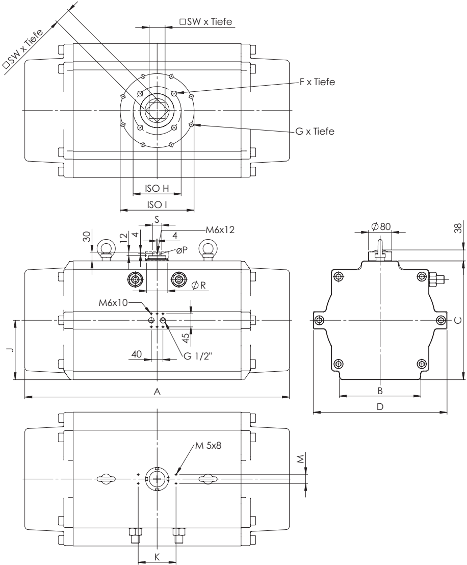
Fig. 13-4 Dimensional drawings for bar-agturn type GD/GS-300 till 400
