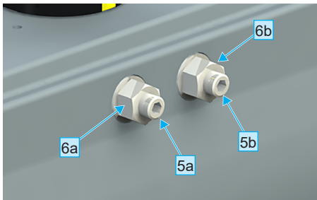
Fig. 6-4 Adjustment of the rotary actuator bar-agturn in details
