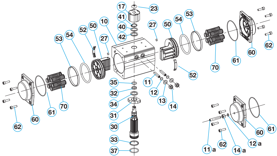
Exploded-view drawing of all individual components of rotary actuator bar-acturn
