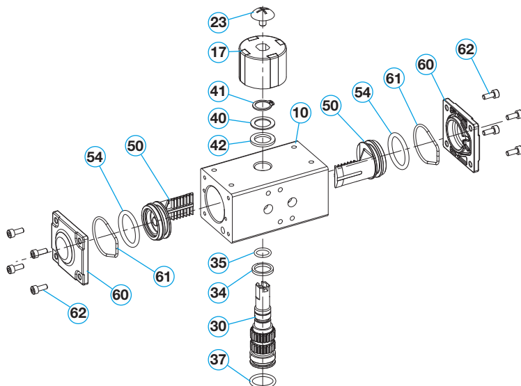
Fig. 9-1 Exploded-view drawing of all individual components of rotary actuator bar-acturn
