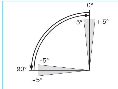
Fig. 6-1 Adjustable mechanical swivel angle range of the bar-acturn version 90° from size GD-040, GD/GS-052 till 400
